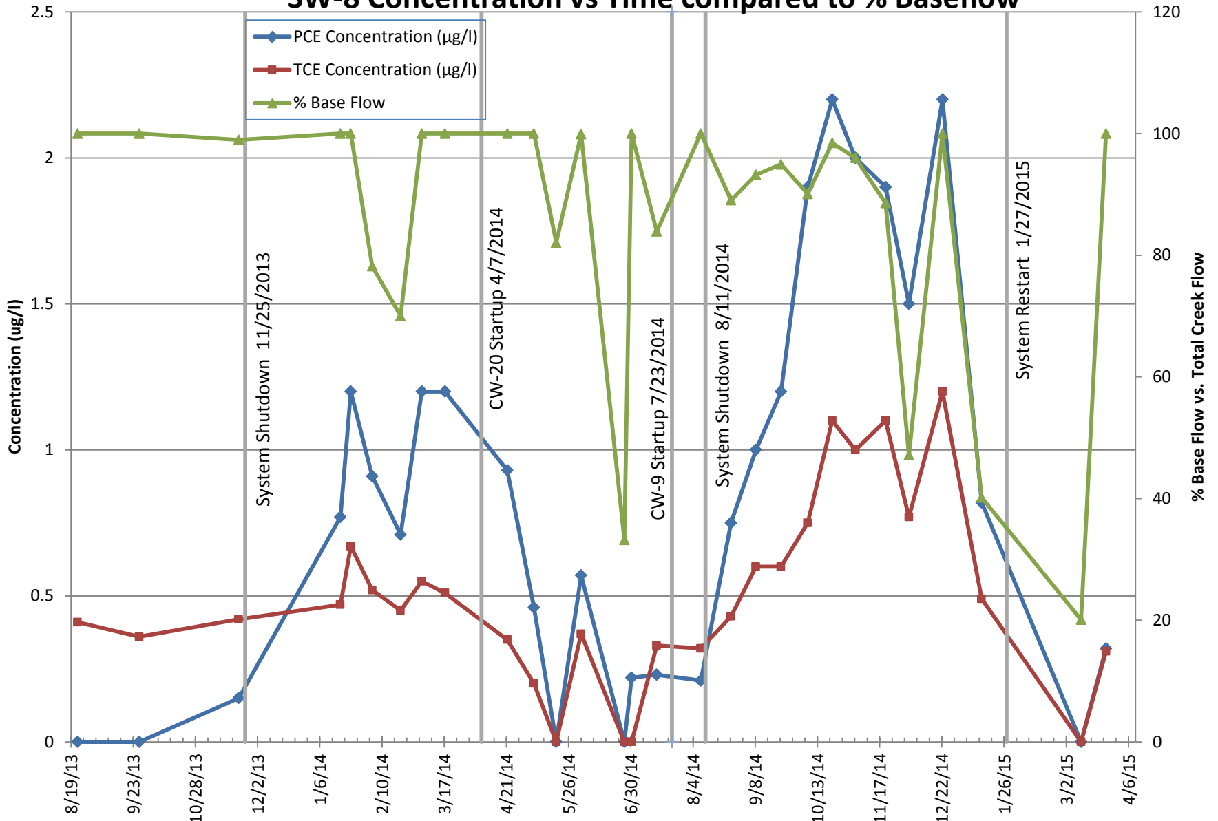
FIGURE 3.5-19 SW-8 Concentration vs Time compared to % Baseflow
